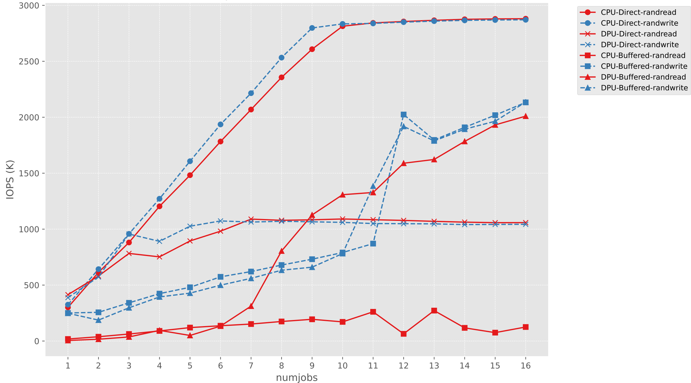
IOPS vs numjobs (CPU vs DPU, Direct vs Buffered)
